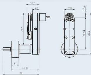
78mm Offset Hi-Lok head
